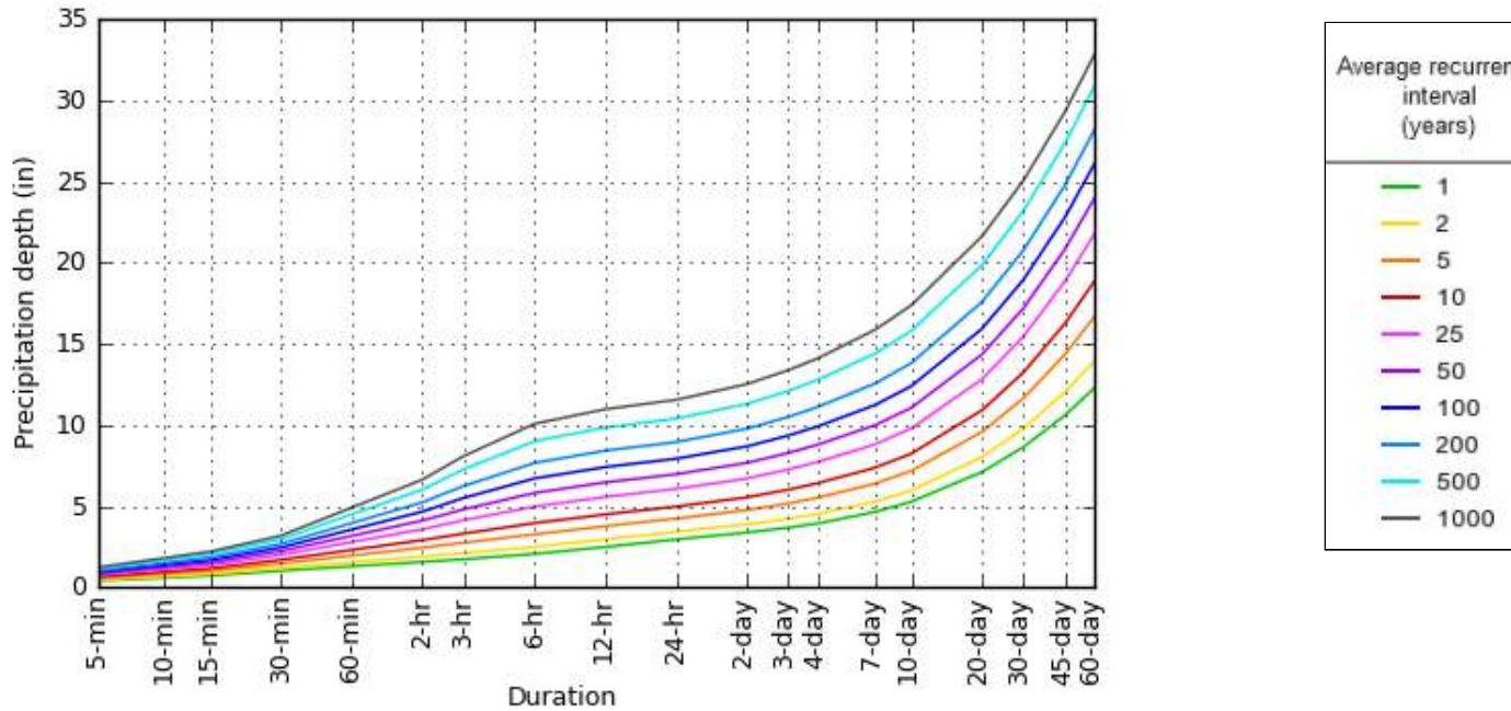
PDS-based depth-duration-frequency (DDF) curves Latitude: 39.5435°, Longitude: -92.6370°
